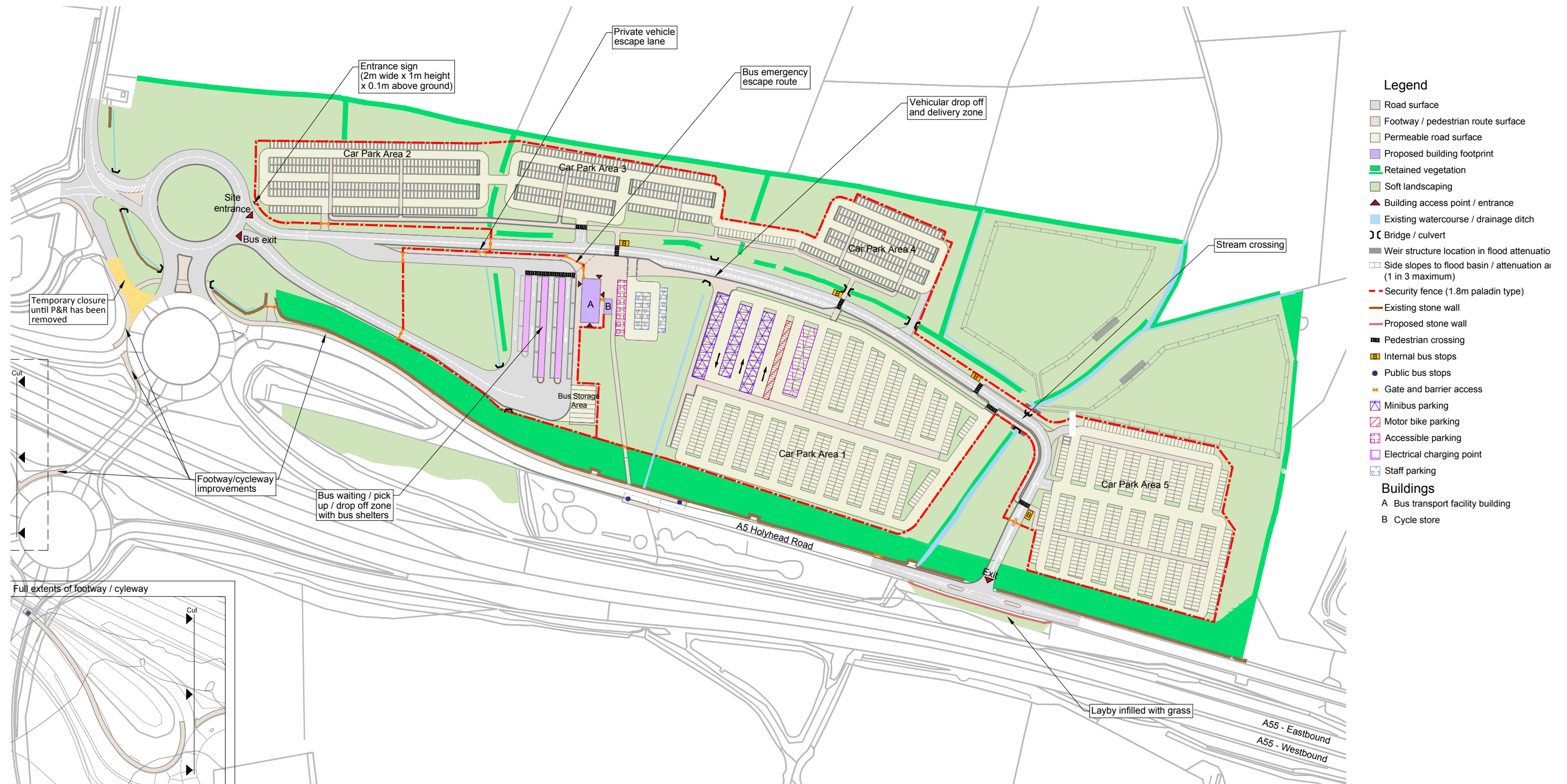
Figure 16 General arrangement plan
