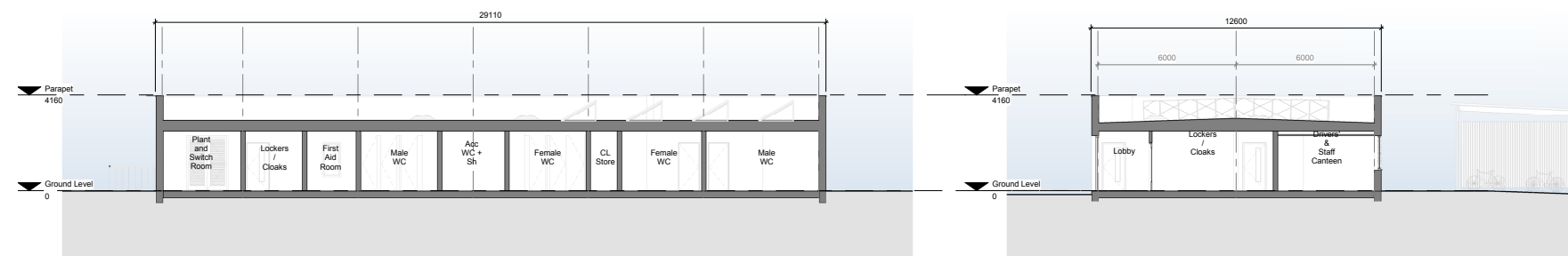
Figure 34 Building sections
