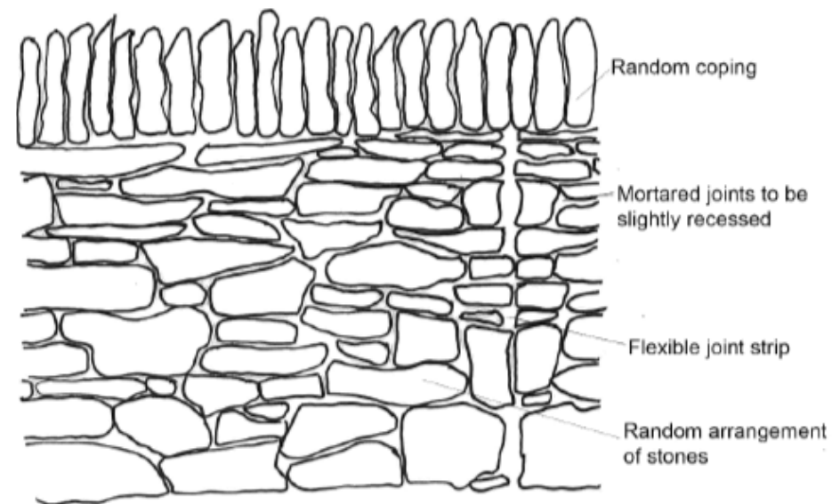
Figure 9 Sketch of proposed stone wall elevation
